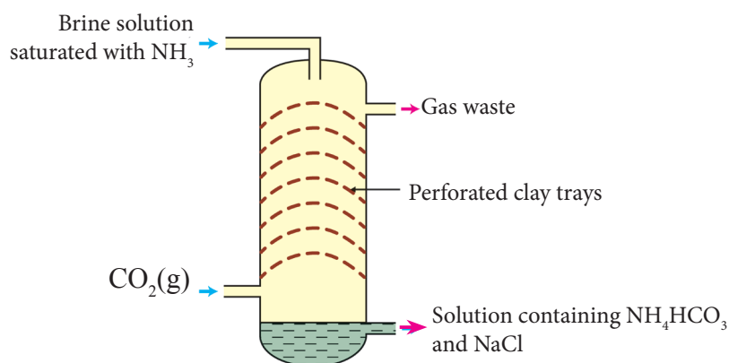
Figure 1.6 Carbonation tower
