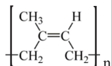
cis -1,4-polyisoprene
