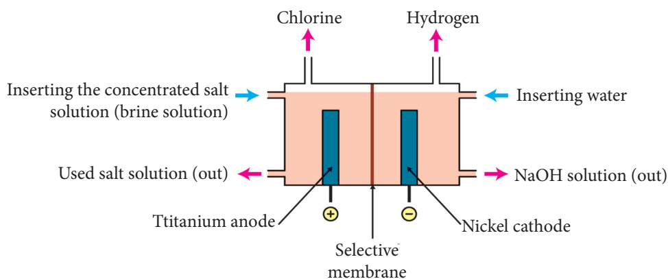
Figure 1.2 Membrane cell
