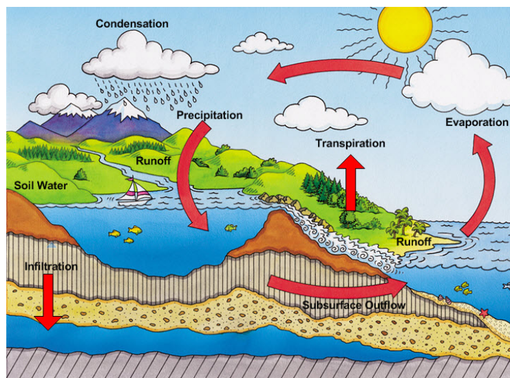
Figure 1.36 Water cycle
